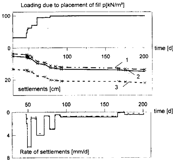
Fig. 2: settlements and rate of settlements in selected measuring points below the embankment.
